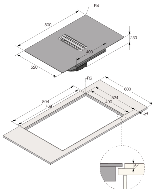
Flush installation
