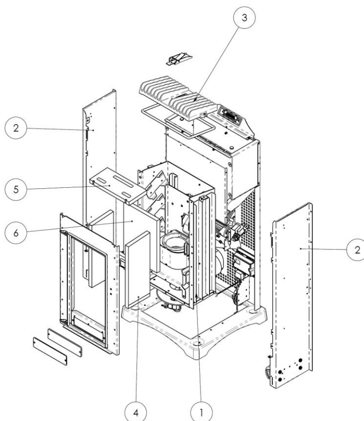
Exploded view of ANTIGUA stove combustion chamber and parts
