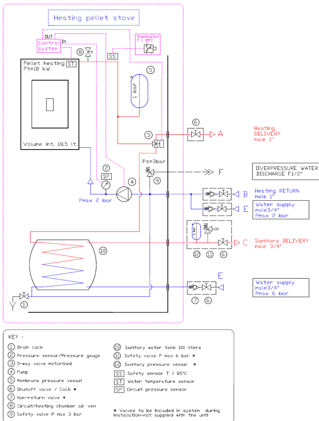
Hydraulic diagram - heating pellet stove 18 kW_04-2015
